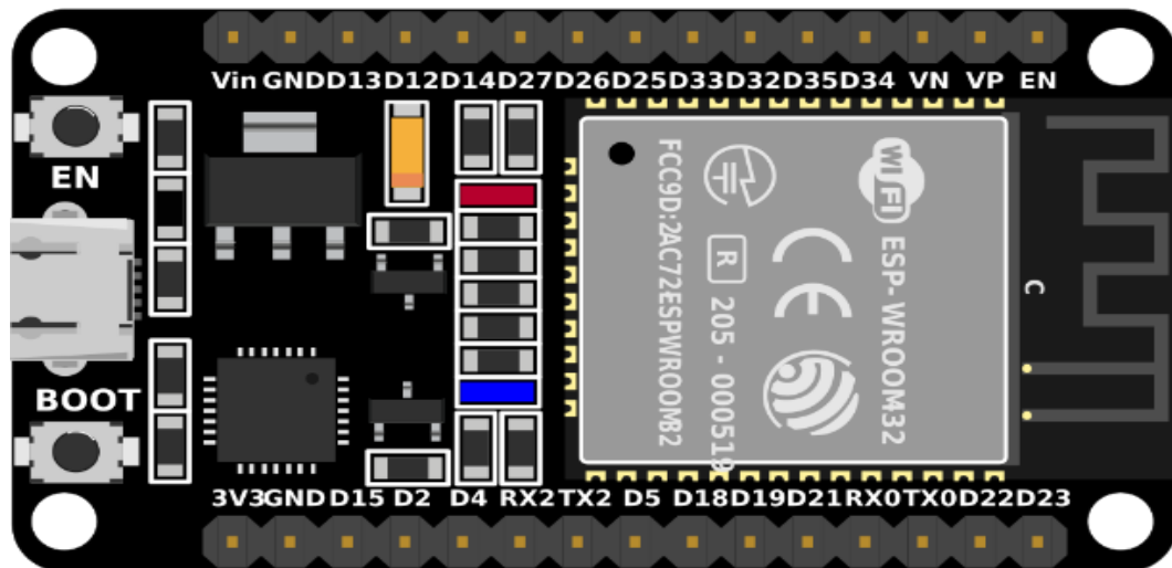
Fig 4.1 ESP32 Microcontroller
