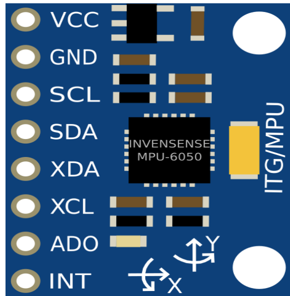
Fig 4.6 MPU6050
